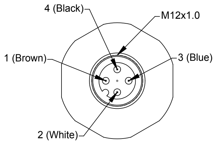
Face View Part #1510-1313006-04 4-Pin Male Eurofast Receptacle
