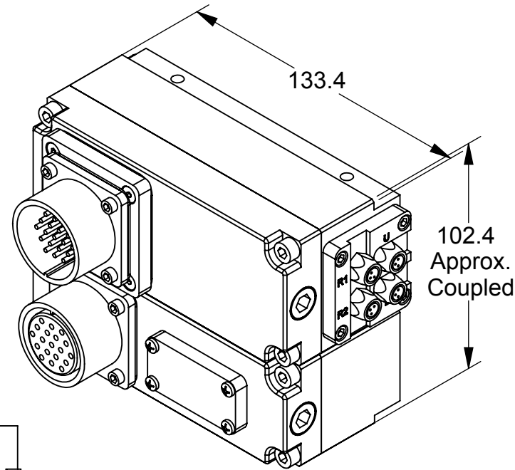
SA12 Master and SA2 Tool Coupled
