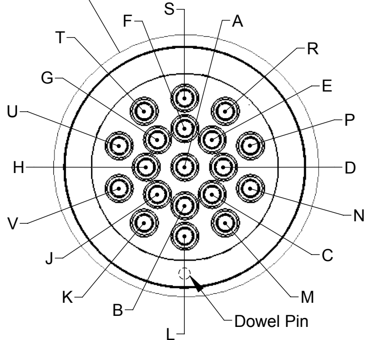
Master Side Pin Block DETAIL A SCALE 2 : 1
