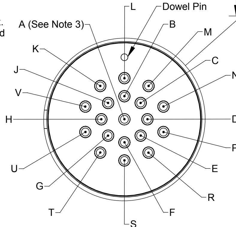
Tool Side Pin Block DETAIL B SCALE 2 : 1
