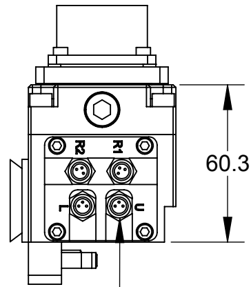
SA12 Master and SA2 Tool Coupled
