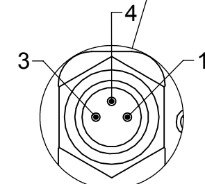
Sensor Connectors 4X Turck MFKS Face View Scale 2:1
