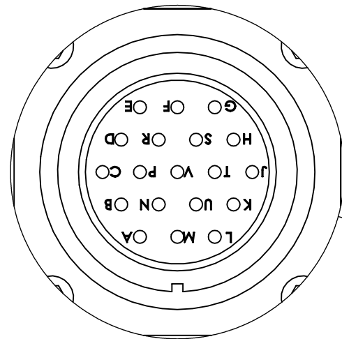
19-Pin Male Connector MS3102E22-14P Face View Scale 3:2
