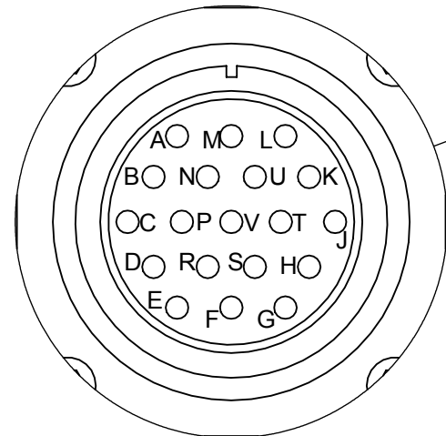
19-Pin Female Connector MS3102E22-14S Face View Scale 3:2
