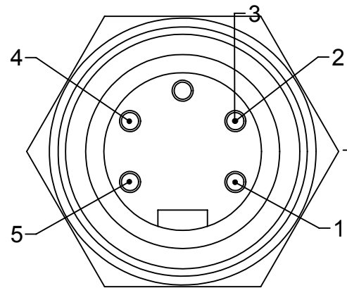
Turck RSFL56-U5229-12 Male Connector SCALE 2:1
