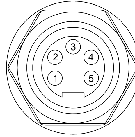
Turck RKFL56-U5515-12 5-Pin Female Connector SCALE 2 : 1 Note Connector Orientation
