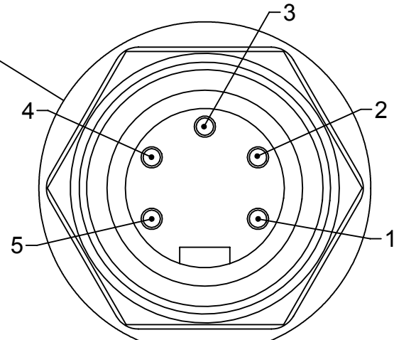
Turck RSFL56-U5229-12 5-Pin Male Connector SCALE 2 : 1 Note Connector Orientation
