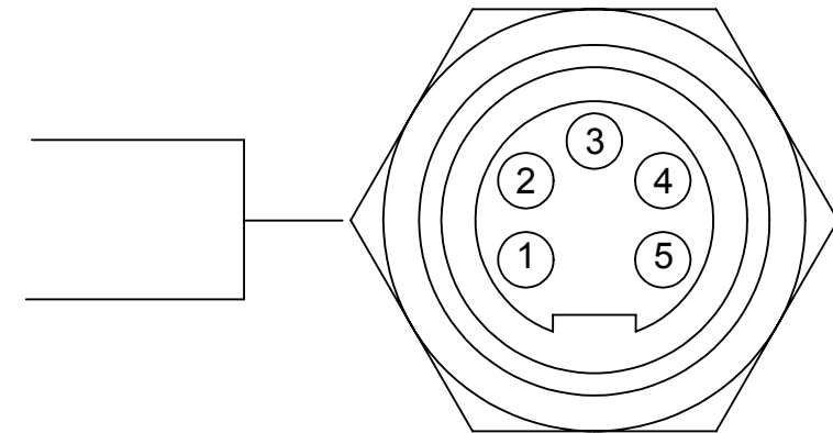
Turck RKFL56-U5515-12 Female Connector SCALE 2:1
