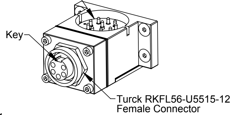
Turck RKFL56-U5515-12 5-Pin Female Connector SCALE 2 : 1 Note Connector Orientation
