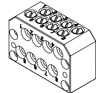
M5 Plugs in Axial Ports (View Rotated)
