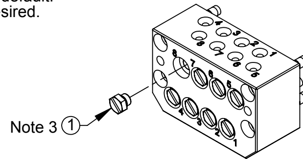
M5 Plugs in Radial Ports (Default Configuration)
