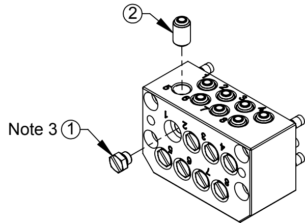
M5 Plugs in Radial Ports (Default Configuration) (View Rotated)
