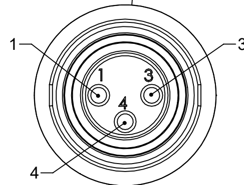
DETAIL D 3-POLE FEMALE CONNECTOR SCALE 4 : 1
