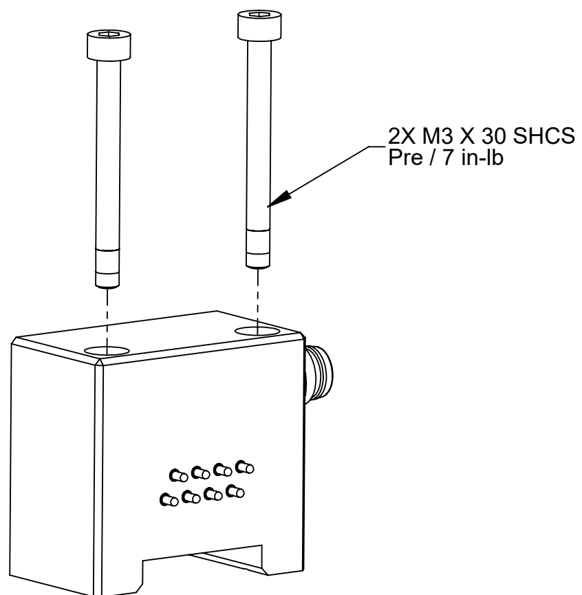
9120-ML8A-M Master Module
