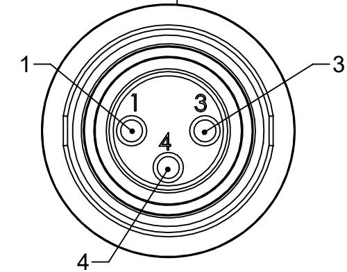
DETAIL E 3-POLE FEMALE CONNECTOR SCALE 4 : 1
