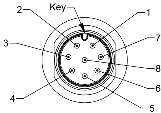
DETAIL C Master 8-Pin Male Connector SCALE 4 : 1
