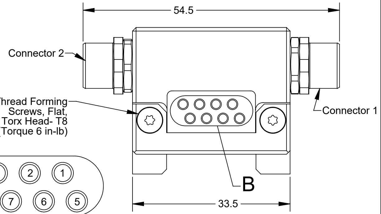
DETAIL B SCALE 4 : 1
