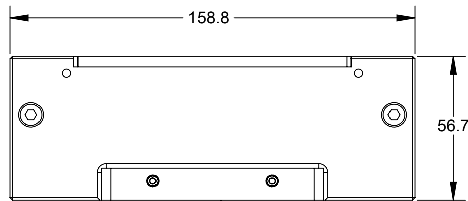
9121-JA2-M Air Adapter (Shown)
