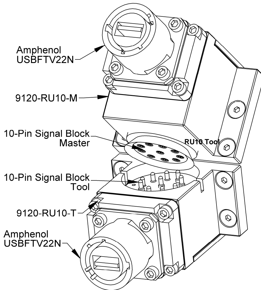
Figure 1.1—Electrical Modules (RU10-M, RU10-T shown)
