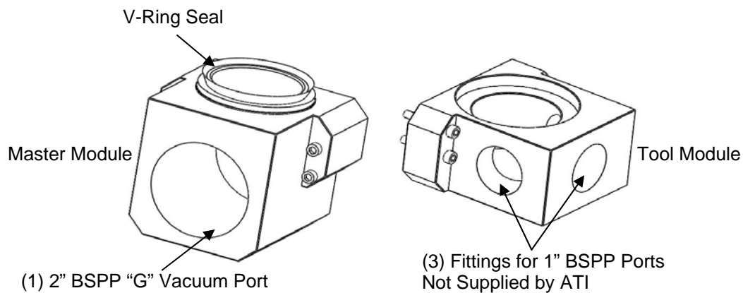
Figure 1.1—Vacuum Module (V200-M-E and V200G1-T-E shown)
