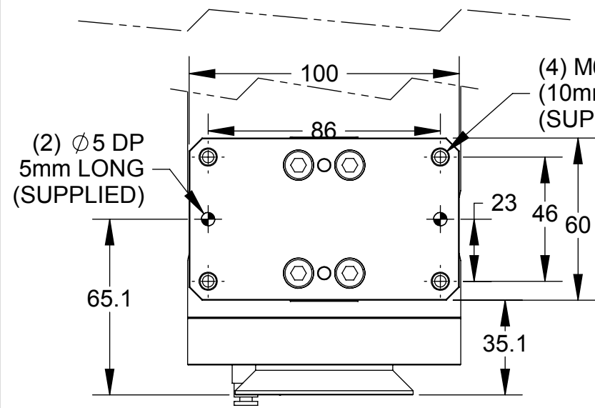
VIEW A-A (9005-50-1029, OPTIONAL BENCH MOUNT ADAPTER)
